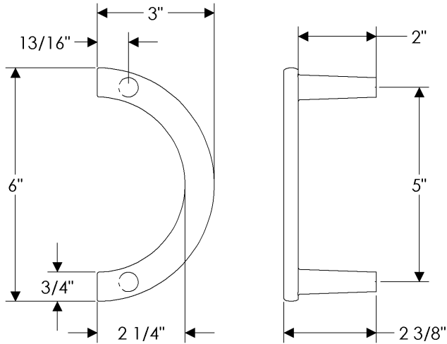
G706 5" Cirque Grip Weight: 1.00 lbs
